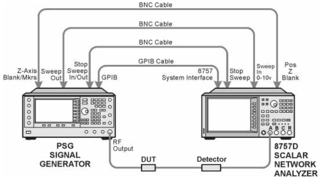
Figure 1-2 Equipment Setup
