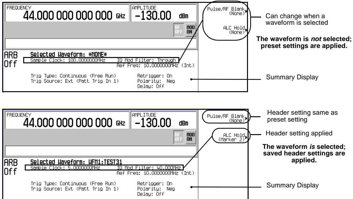
Figure 2-8 File Header Settings
