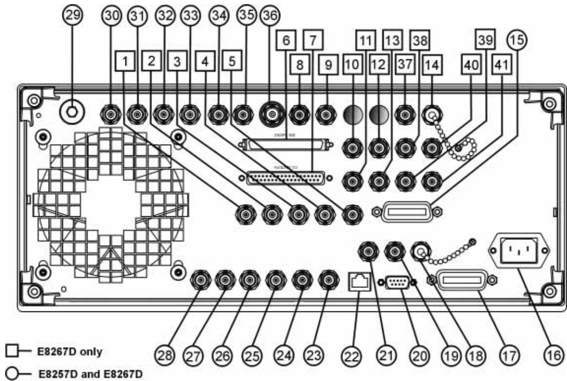
Figure 3-4 Option 1EM Rear Panel Diagram
