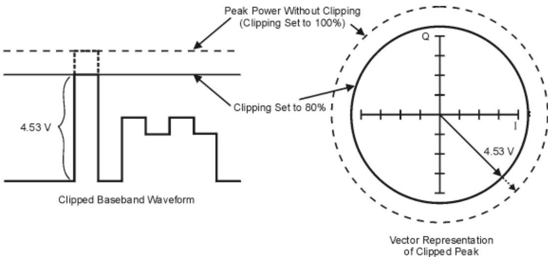
Figure 2-14 Circular Clipping
