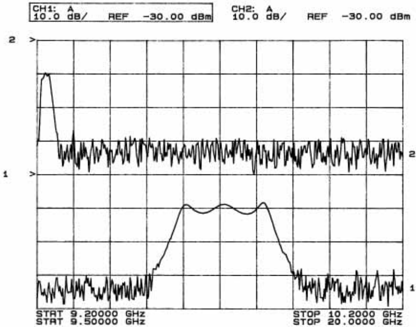
Figure 1-6 Alternating Sweeps on 8757D
