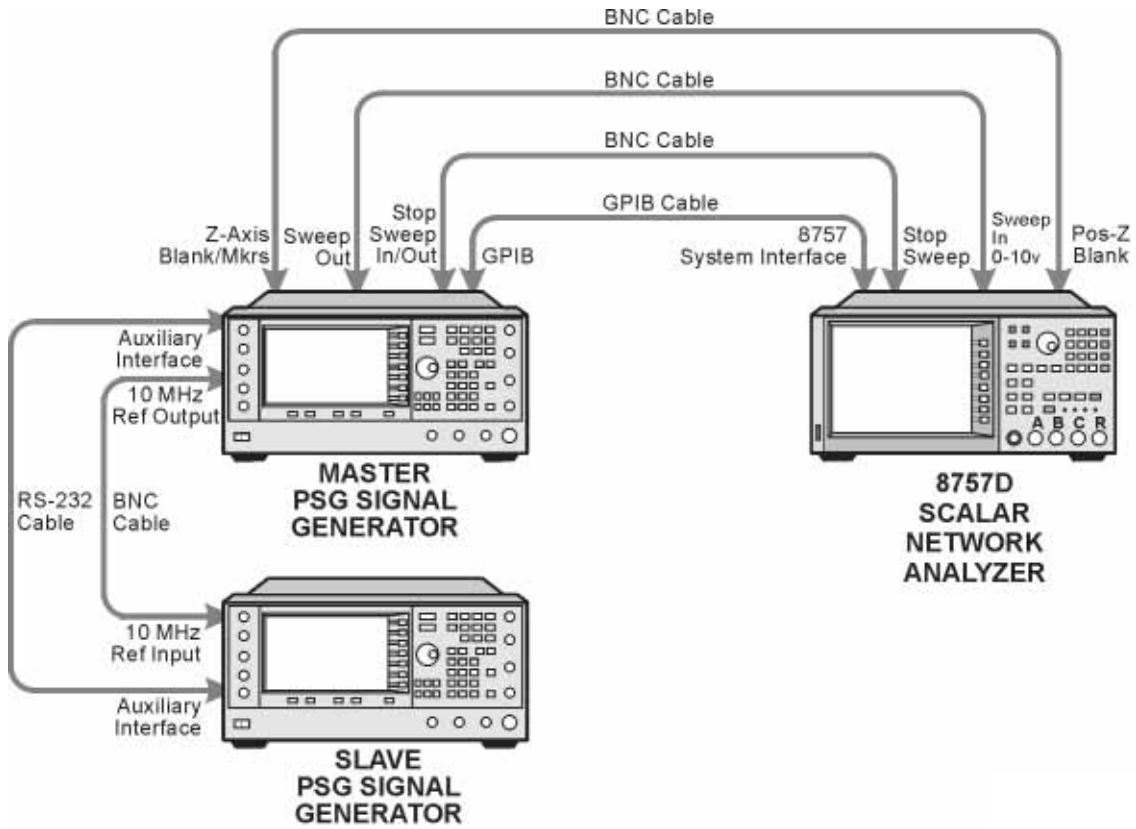
Figure 1-7 Master/Slave Equipment Setup
