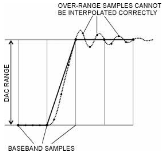
Figure 2-18 Waveform Overshoot
