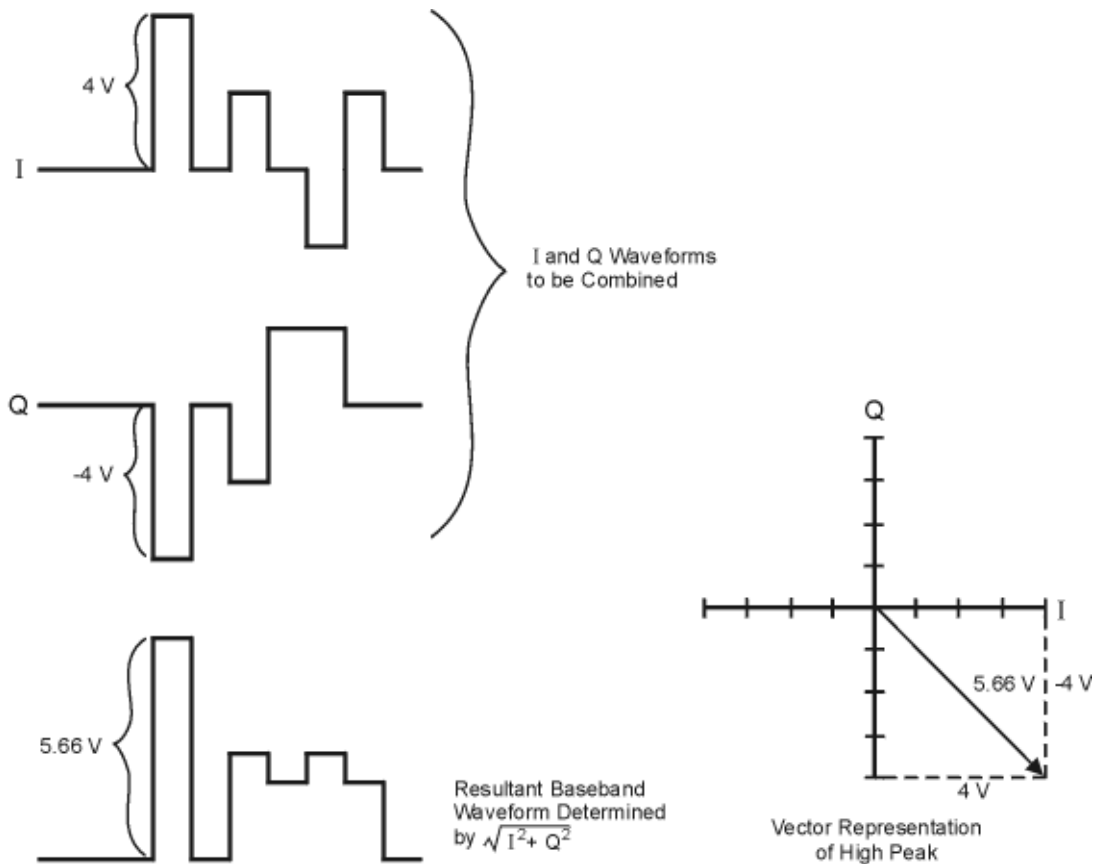
Figure 2-11 Combining the I and Q Waveforms
