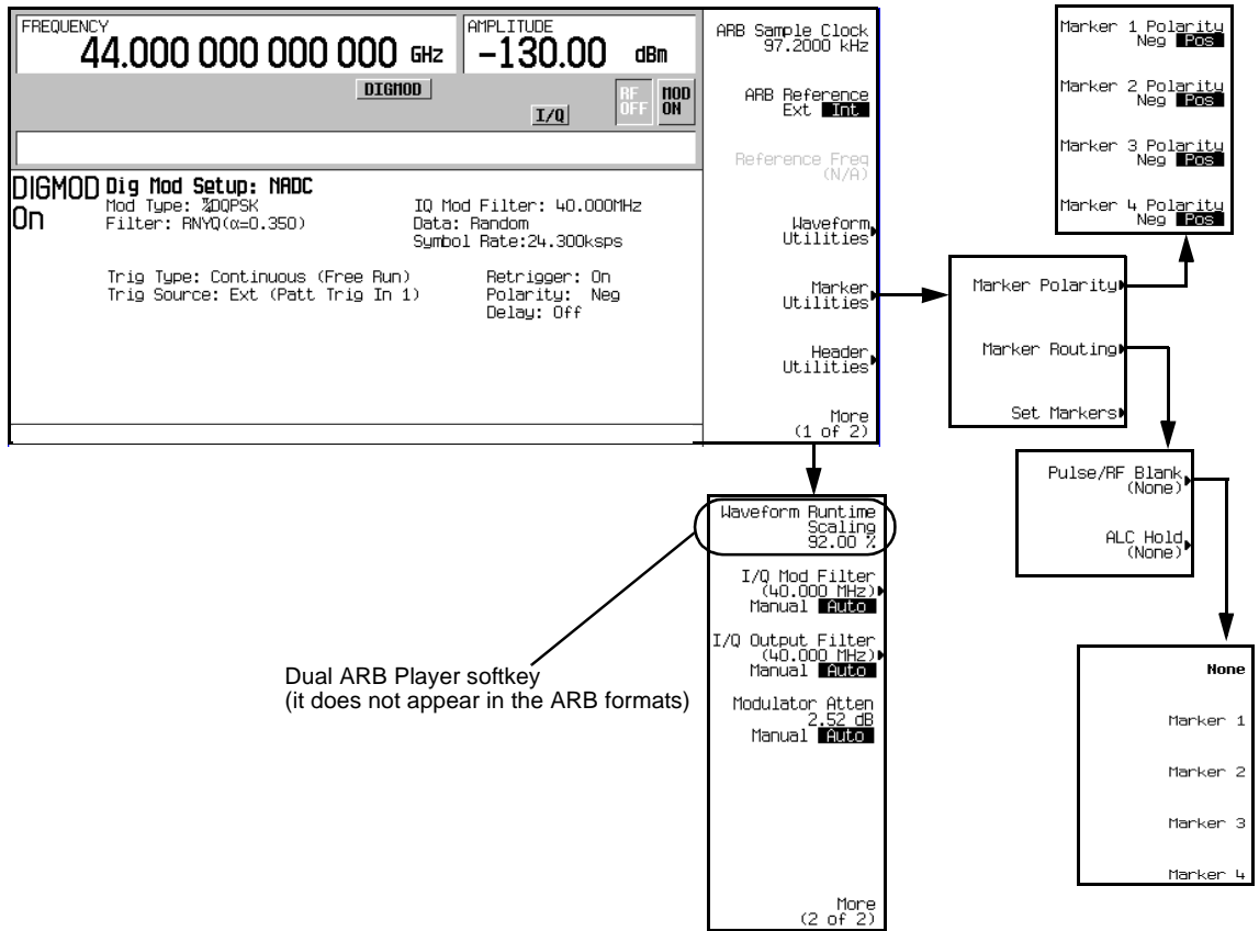
Figure 2-3 ARB Setup Softkey Menu and Marker Utilities
