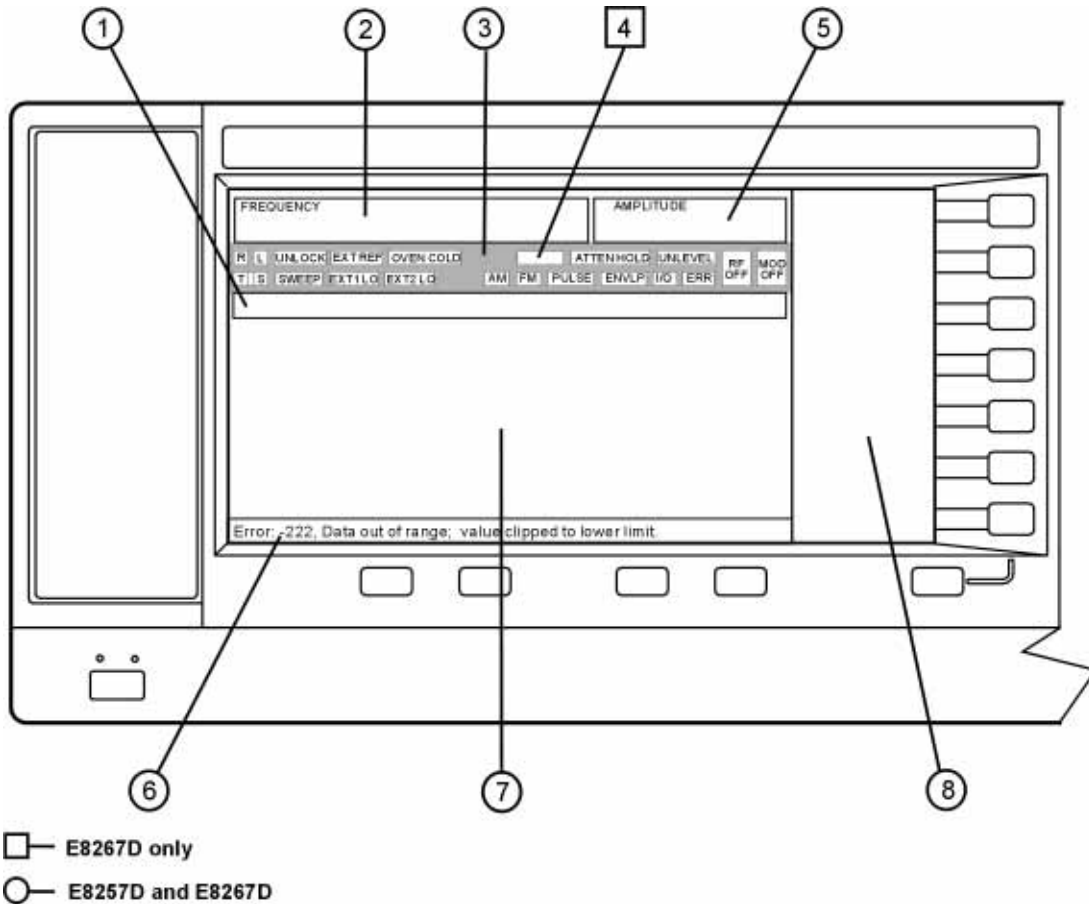
Figure 3-2 Front Panel Display Diagram
