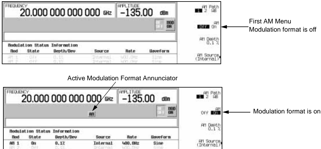
Figure 1-9 Example of AM Modulation Format Off and On
