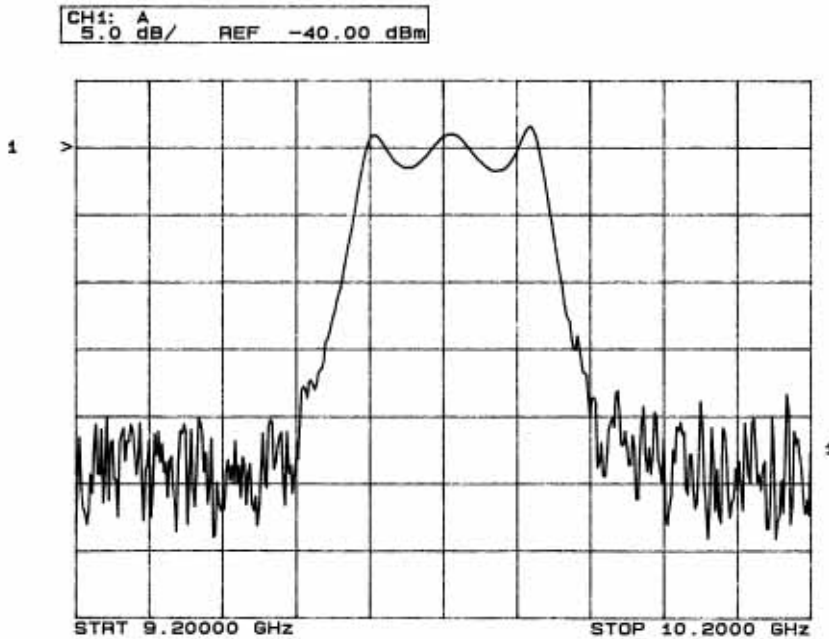
Figure 1-3 Bandpass Filter Response on 8757D
