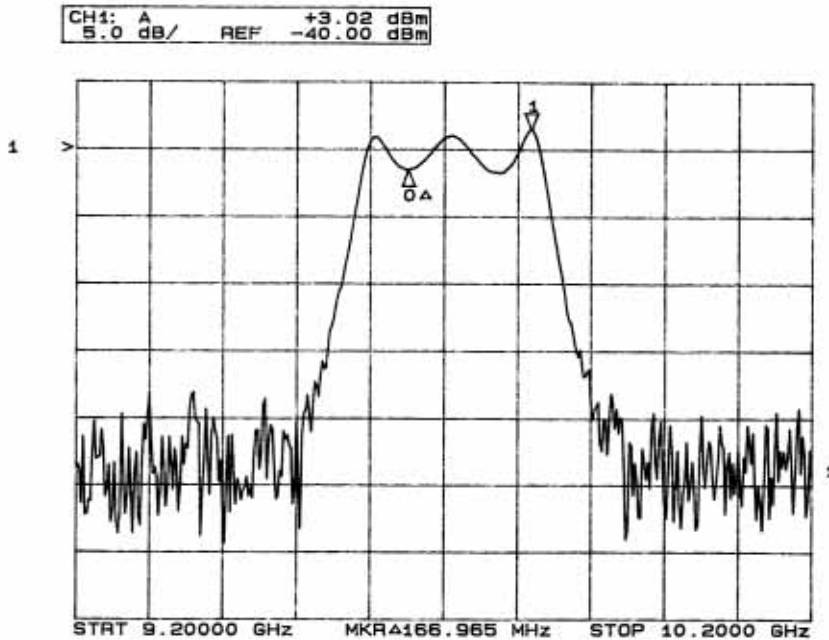
Figure 1-5 Delta Markers on 8757D
