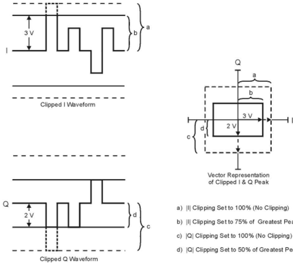
Figure 2-15 Rectangular Clipping
