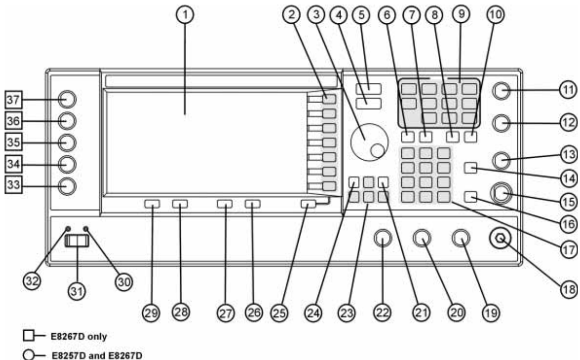
Figure 3-1 Front Panel Diagram (E8267D PSG Vector Signal Generator)
